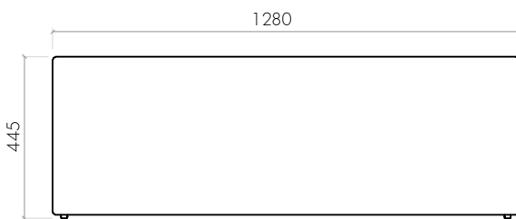
CU_32_128_45_I • THE CUBE • L 1280 x W 320 x H 445
