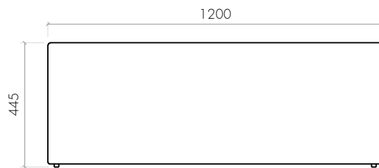
CU_40_120_45_I • THE CUBE • L 1200 x W 400 x H 445
